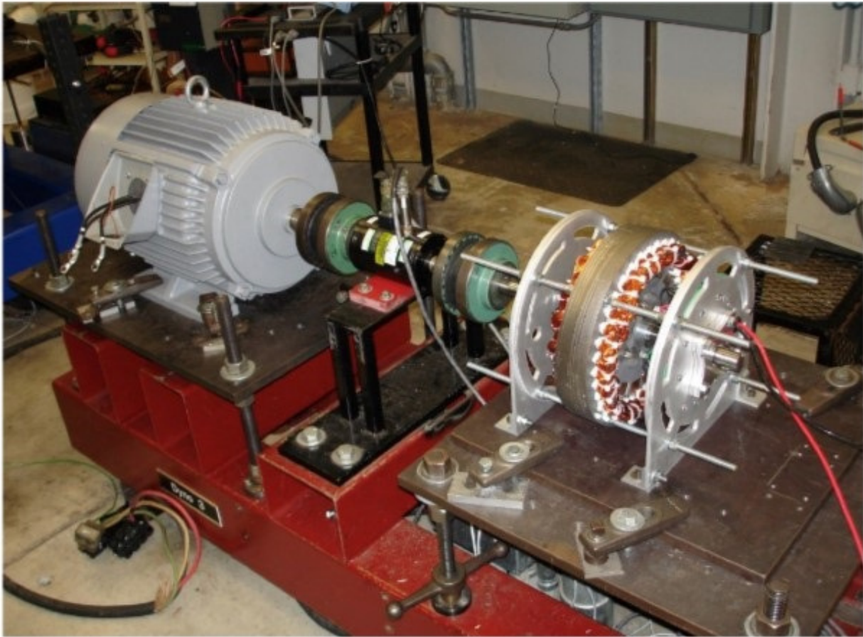
Figure 2: Permanent Magnet generator on dynamometer
