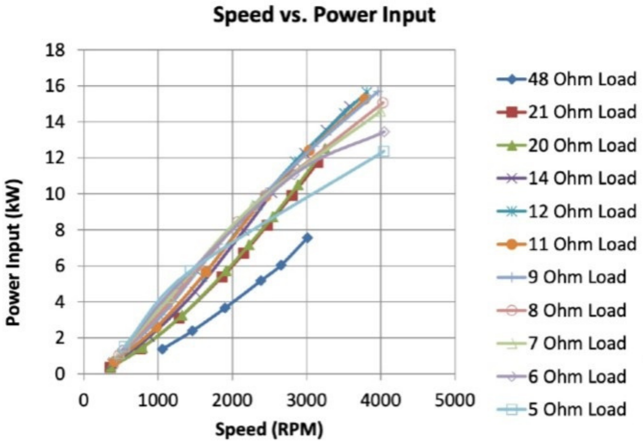
Figure 7: Speed vs. Power input at various Loads
