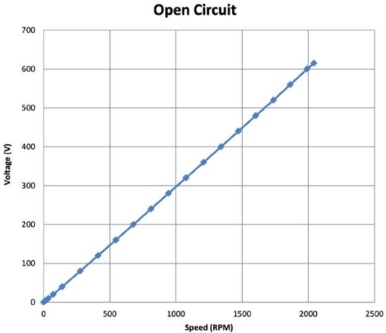
Figure 4: Voltage-speed characteristics at open circuit
