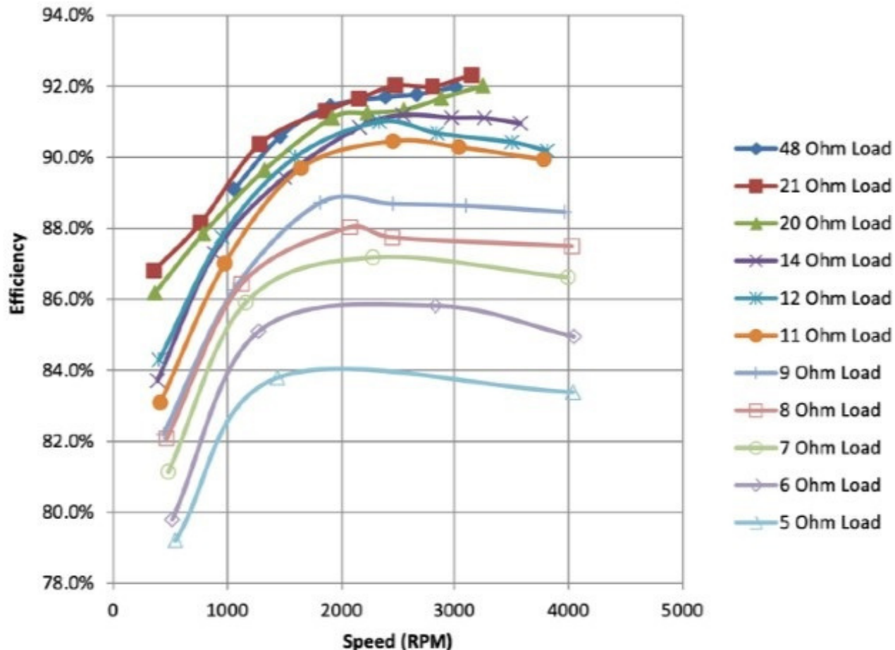
Figure 6: Speed vs. Efficiency at various Loads
