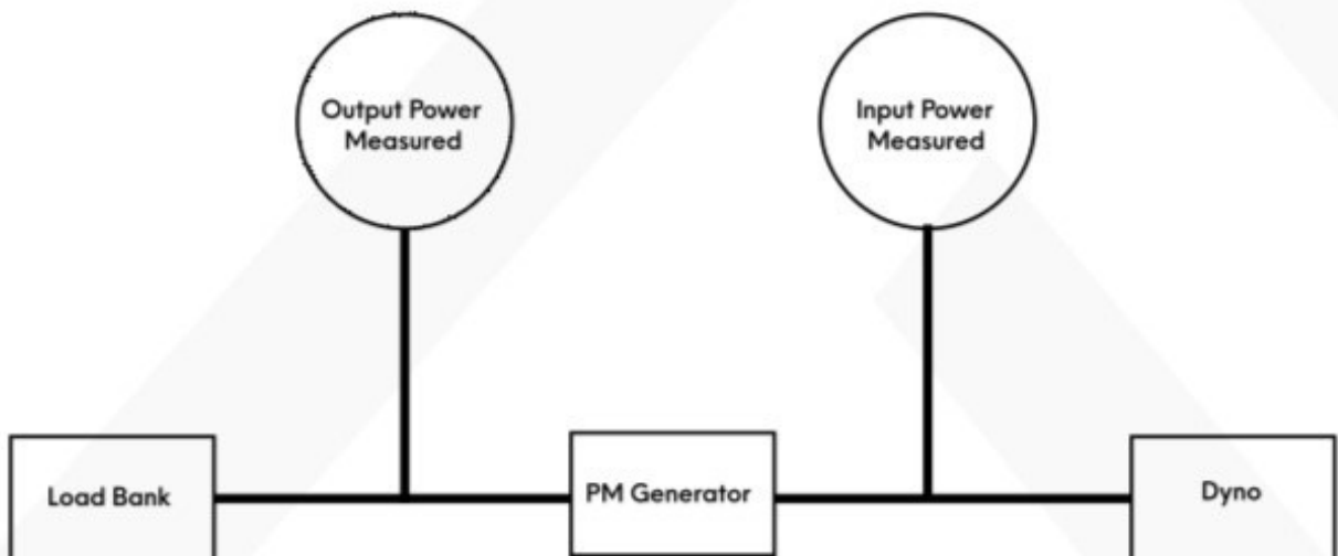
Figure 3: Schematic of the test setup
