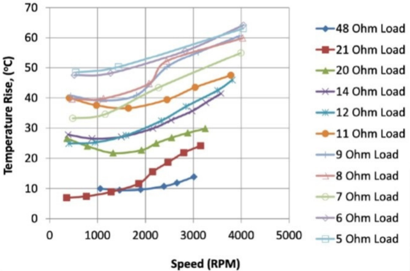
Figure 8: Speed vs. temperature rise over ambient at various Loads
