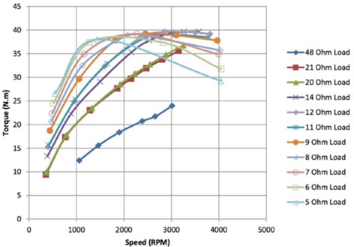
Figure 5: Speed vs. Torque at various Loads
