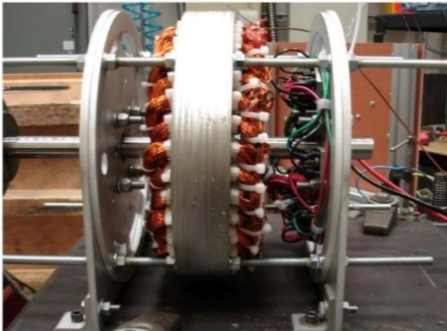
Figure 1: Permanent Magnet generator
